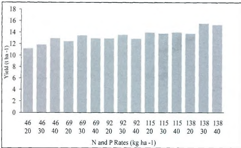
Figure 3. Effect of N and P rates rate on marketable green pod yield
