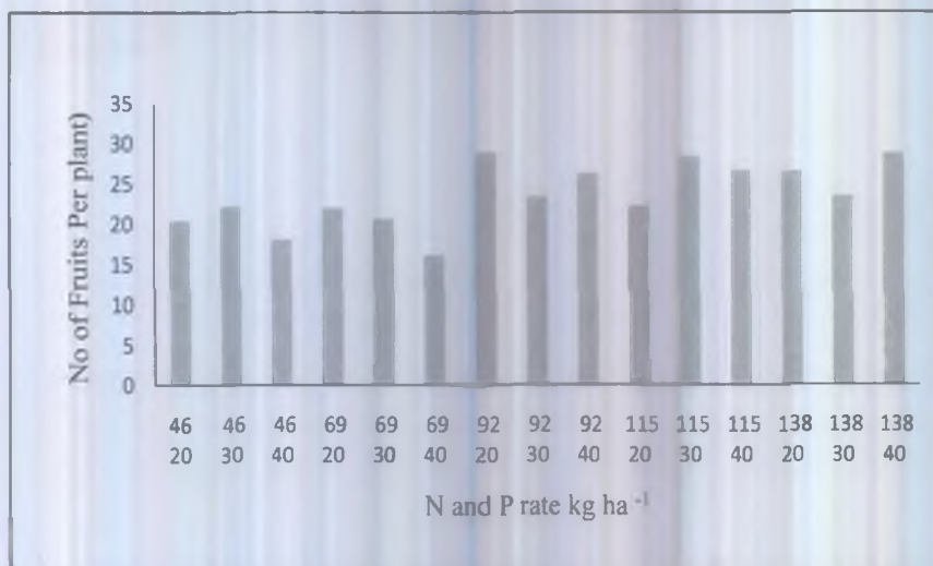
Figure 2. Effect of Nitrogen and Phosphorus Fertilizers on number of fruits per plant
