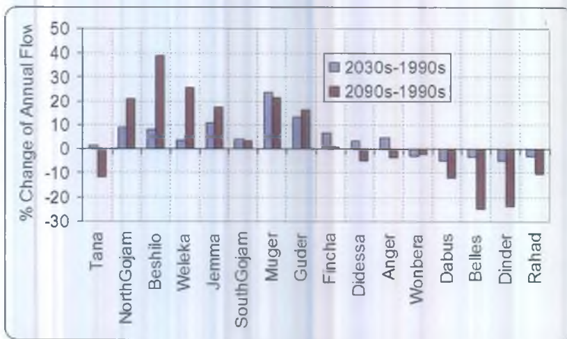
Figure 3. Projected changes in annual flow amounts in the watersheds of the Blue Nile River Basin
