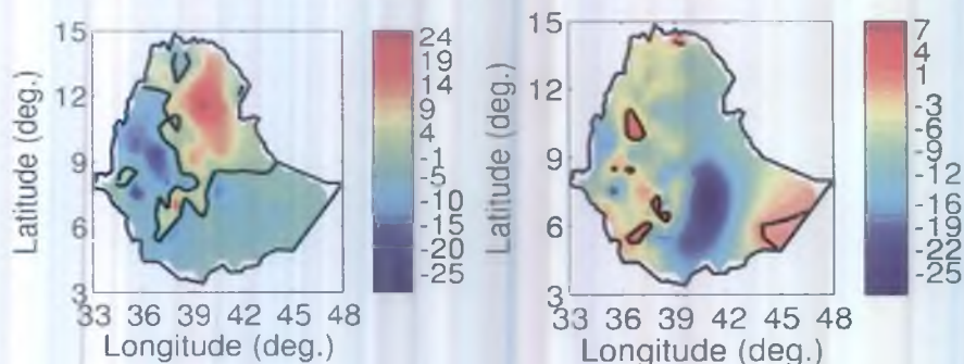
Figure 1. The linear seasonal rainfall trend (mm/decade) over 1978-2007 period for summer (left) and spring (right) based on gridded rain gauge observations (Source: Unpublished work by this author).
