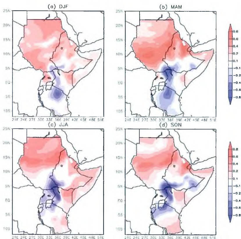
Figure 2. The linear seasonal mean temperature trend (°C/decade) over 1981-2014 period for (a) winter (DJF); (b) spring (MAM); (c) summer (JJA) and (d) autumn (SON) based ERA-Interim temperature data (Source: Unpublished work by this author).
