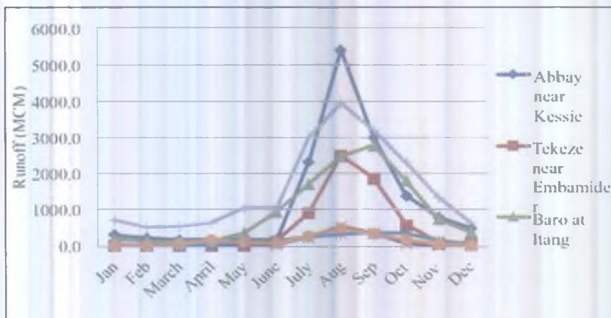
Figure 2. Flow characteristics of some of the Ethiopian rivers, showing very high seasonality.
